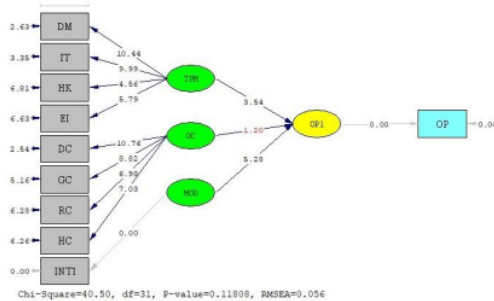
Figure 6. SEM of second step with interaction (t-value)
