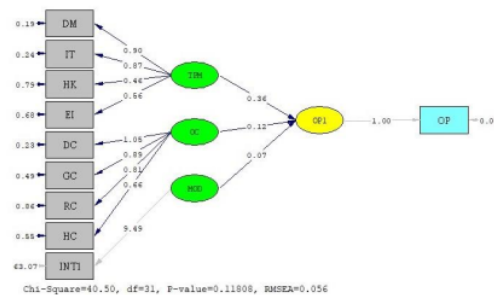
Figure 7. SEM of second step with interaction (coefficient of estimation)
