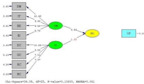
Figure 4. SEM of first step without interaction (t-value)
